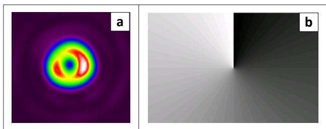
FIGURE 11: (a) Image of a vortex beam with l = 1 , showing the intensity distribution. (b) A greyscale phase pattern encoded with an azimuthal phase was used to convert the incoming Gaussian laser beam to the vortex beam.
