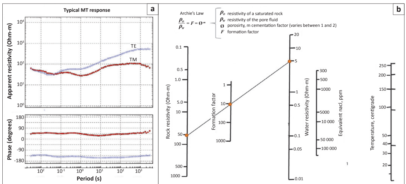
FIGURE 2: (a) An example of magnetotelluric (MT) data showing the transverse electric (TE) and transverse magnetic (TM) apparent resistivity and phase responses plotted against increasing period, the latter being a proxy for increasing depth. (b) The porosity–resistivity–salinity nomogram is used to estimate porosity percentage from bulk resistivity measurements.
