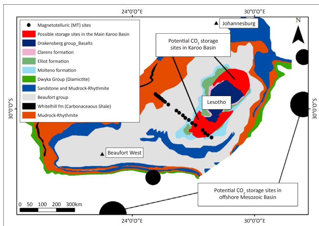
FIGURE 1: Map showing the distribution of potential onshore and offshore CO 2 storage sites and the locations of magnetotelluric stations in the Karoo Basin.
