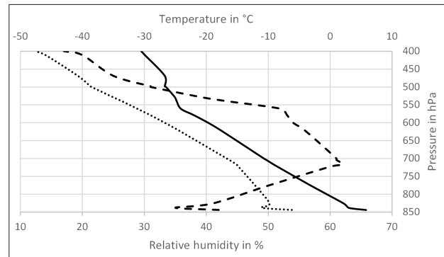
Figure 6: The vertical profile of temperature (solid), dew point temperature (dotted) and relative humidity (dashed) as obtained from upper air ascent at Irene on 7 August 2012 at 1200 UTC.
