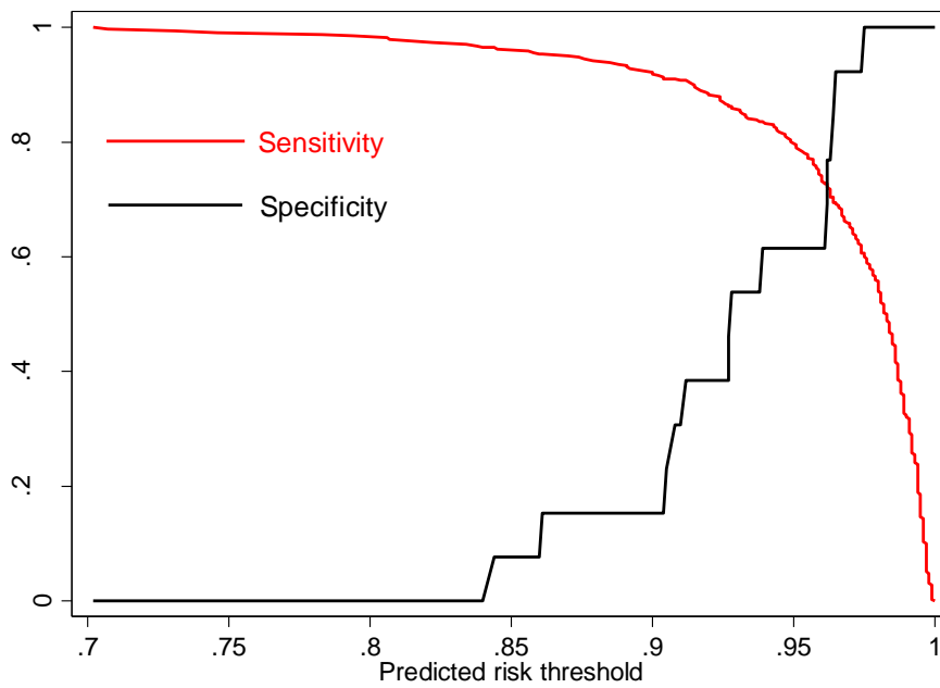
Supplementary figure 4: Estimated sensitivity and specificity by risk threshold (Modelling group, 361 deceased claimants).
