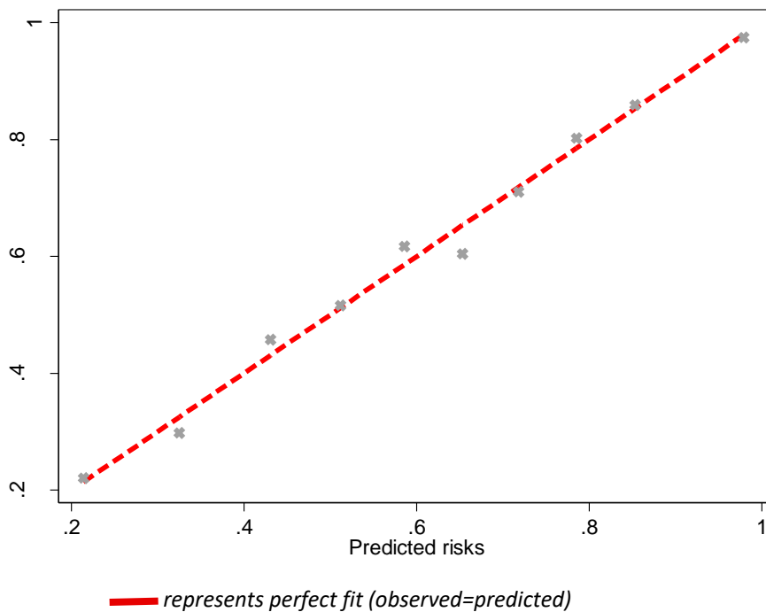
Supplementary figure 2: Observed vs predicted risk deciles.
