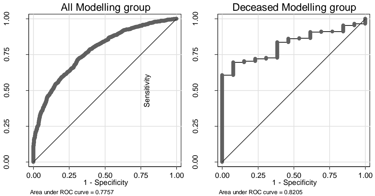
Supplementary figure 1: Receiver operating characteristic (ROC) curves for the final model.
