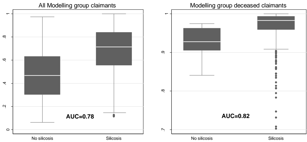
Supplementary figure 3: Predicted risk of silicosis by true silicosis status.
