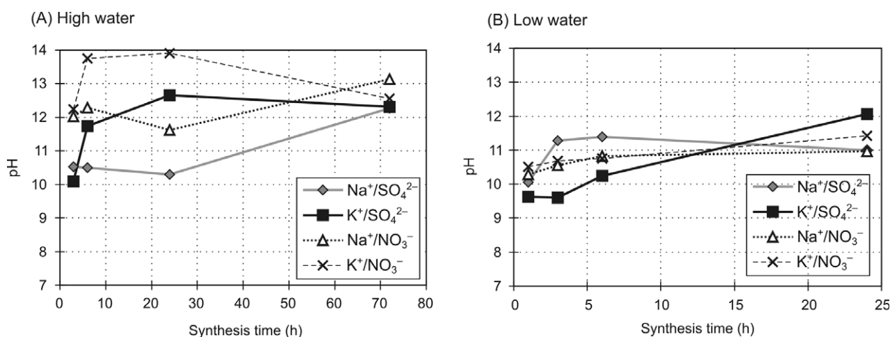
Fig. 2. pH for different combinations of anions and cations.
