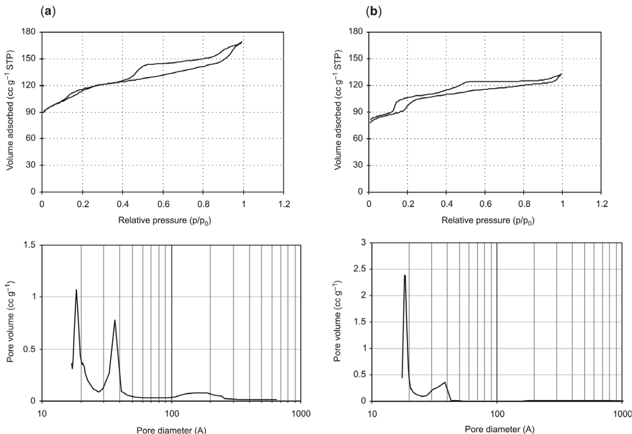
Fig. 5. Capillary condensation and BJH desorption plots for (a) Na^+/SO_4^{2-} and (b) K^+/SO_4^{2-} combinations in high water.
