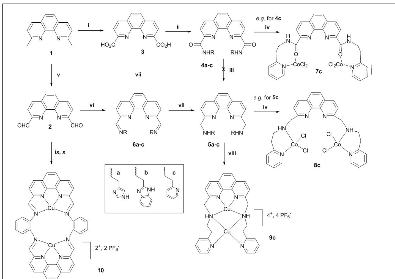
Reagents: (i) 80% HNO_3 ; (ii) RNH_2 , CDI; (iii) LiAlH_4 , THF; (iv) CoCl_2 \cdot 6H_2O , DMF; (v) SeO_2 , 1,4-dioxane; (vi) RNH_2 , CHCl_3 ; (vii) NaBH_4 , MeOH; (viii) Cu(MeCN)_4PF_6 , DMF; (ix) 1,2-diaminobenzene, MeOH; and (x) Cu(MeCN)_4PF_6 , DMF, N_2 .
